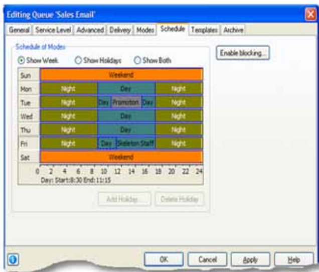
Figure 1. Queue Schedule
